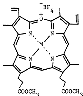
(14) M = Fe(II)·Py 2
