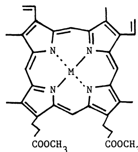
(16) M = Fe(II)·(TsCH 2 NC) 2
