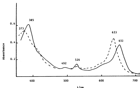
Fig. 1. Absorption spectra ( \text{CH}_2\text{Cl}_2 ) of the (—) bis(pyridine) (4) ( 1.4\times 10^{-5}\text{M} ) and (---) bis( \text{TsCH}_2\text{NC} )iron(II) 5-oxamesoporphyrin IX dimethyl ester (5).
