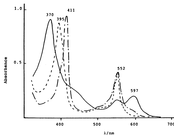
Fig. 2. Absorption spectra (1% pyridine- \text{CH}_2\text{Cl}_2 , v/v) of 5-azamesoporphyrin IX iron(III) (10) (—) ( 2.5\times 10^{-5}\text{M} ) and bis(pyridine) (11) (---) and bis( \text{TsCH}_2\text{NC} )iron(II) 5-azamesoporphyrin IX dimethyl ester (12) (-·-·-).
